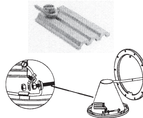
ST-355 ANTI-ELECTROLYSIS ZINC UNDERWATER LIGHT ANODE Contains 1 Anode, 1 Copper Lug, 1 #8 Copper Wire and 1 1/4-20 Hex Nut
