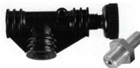
122092 BLACK AIR RELIEF VALVE TO FIT PENTAIR FILTERS Replaces: 154687
