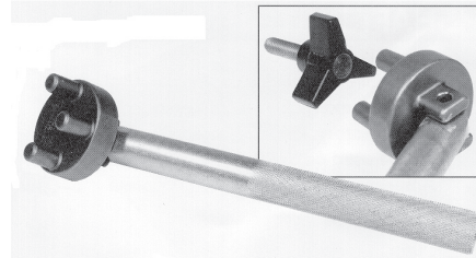
ST-346 CLAMP KNOB WRENCH 9" Long and 3 lbs.
