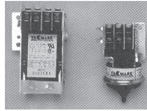
SW-550 UNIVERSAL PRESSURE SWITCH FOR GAS AND ELECTRIC POOL HEATERS Includes: 1 Barb Fitting, one 1/4" and one 3/16" Compression Fitting
