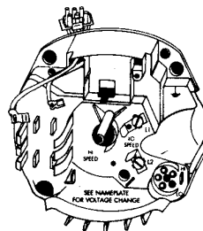
301324 BASE PLATE-INCLUDES QUICK DISCONNECT PLUG AND TERMINALS Single Speed
